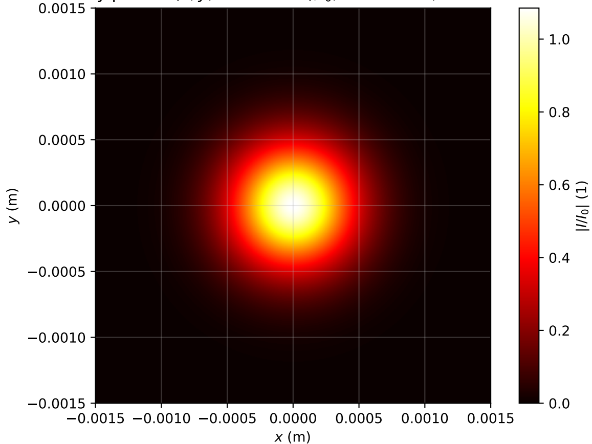
Intensity profile I(x, y, z = 0.478m)/I_0 , P_{in}=0.7P_{cr} , artificial time
